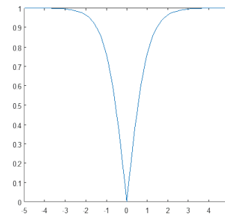
Figure 10: Plot of absolute of hyperbolic tangent function
